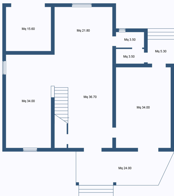
Piano terra
